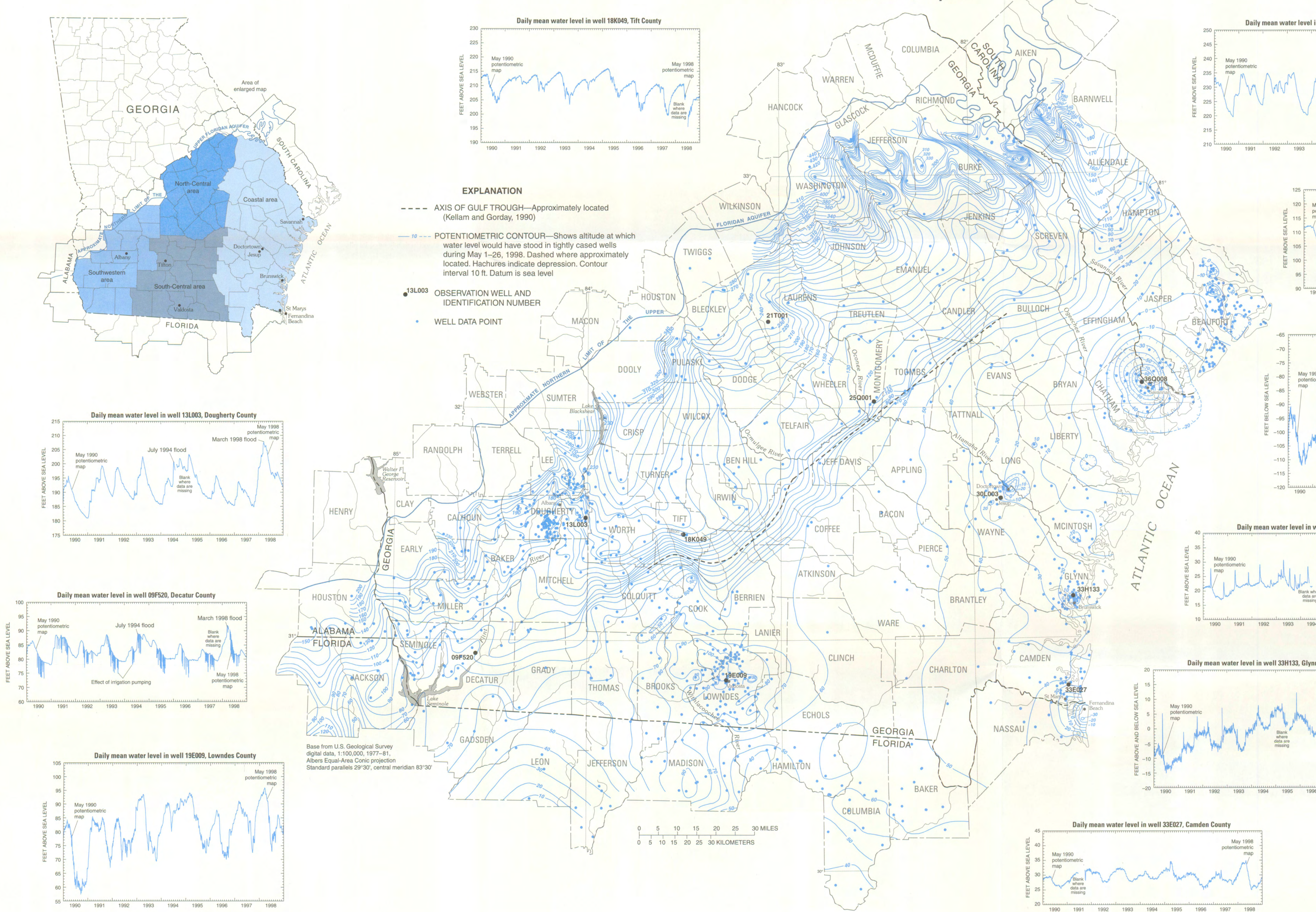
Potentiometric surface, May 1998
