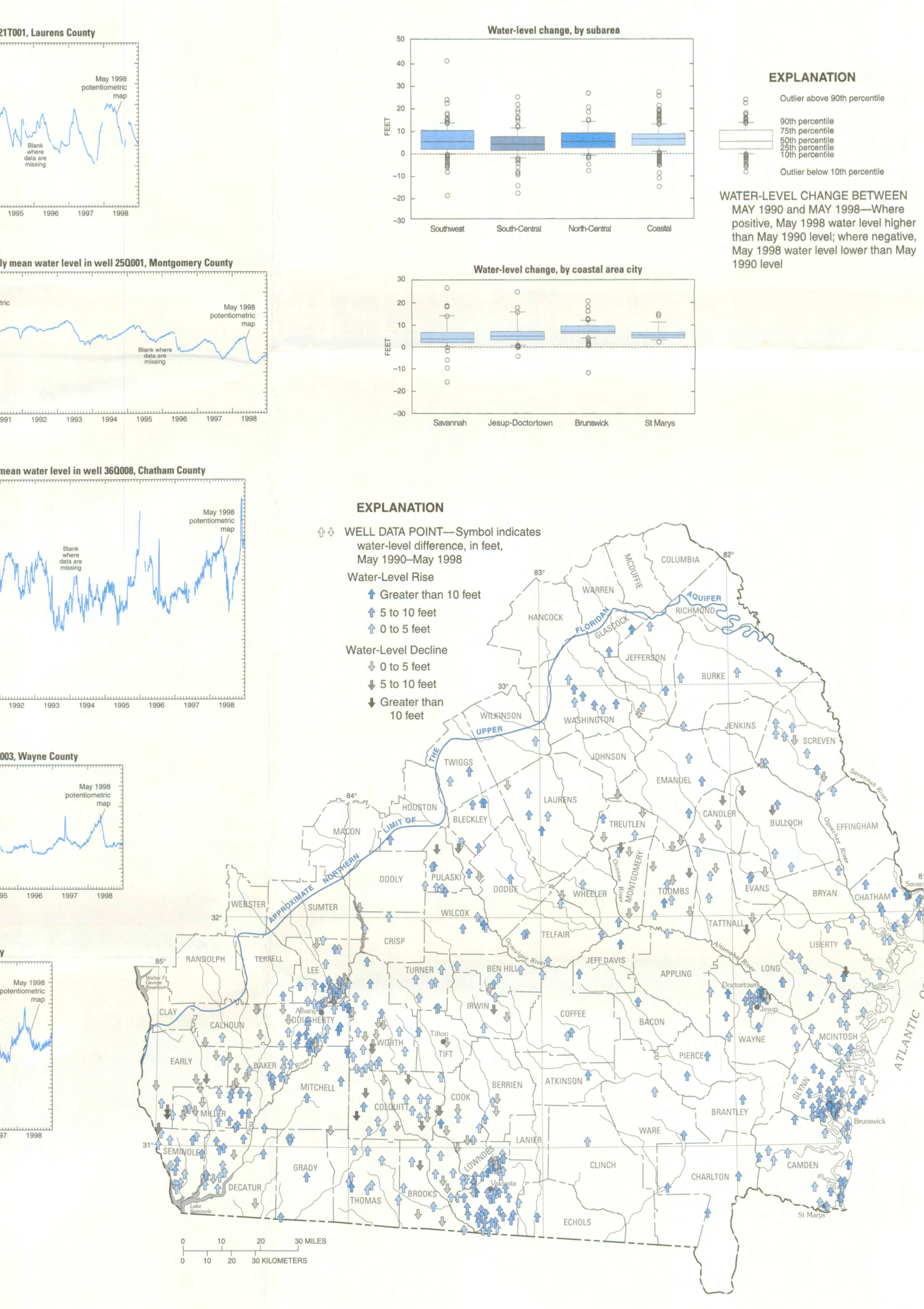
Water-level change, May 1990-98
