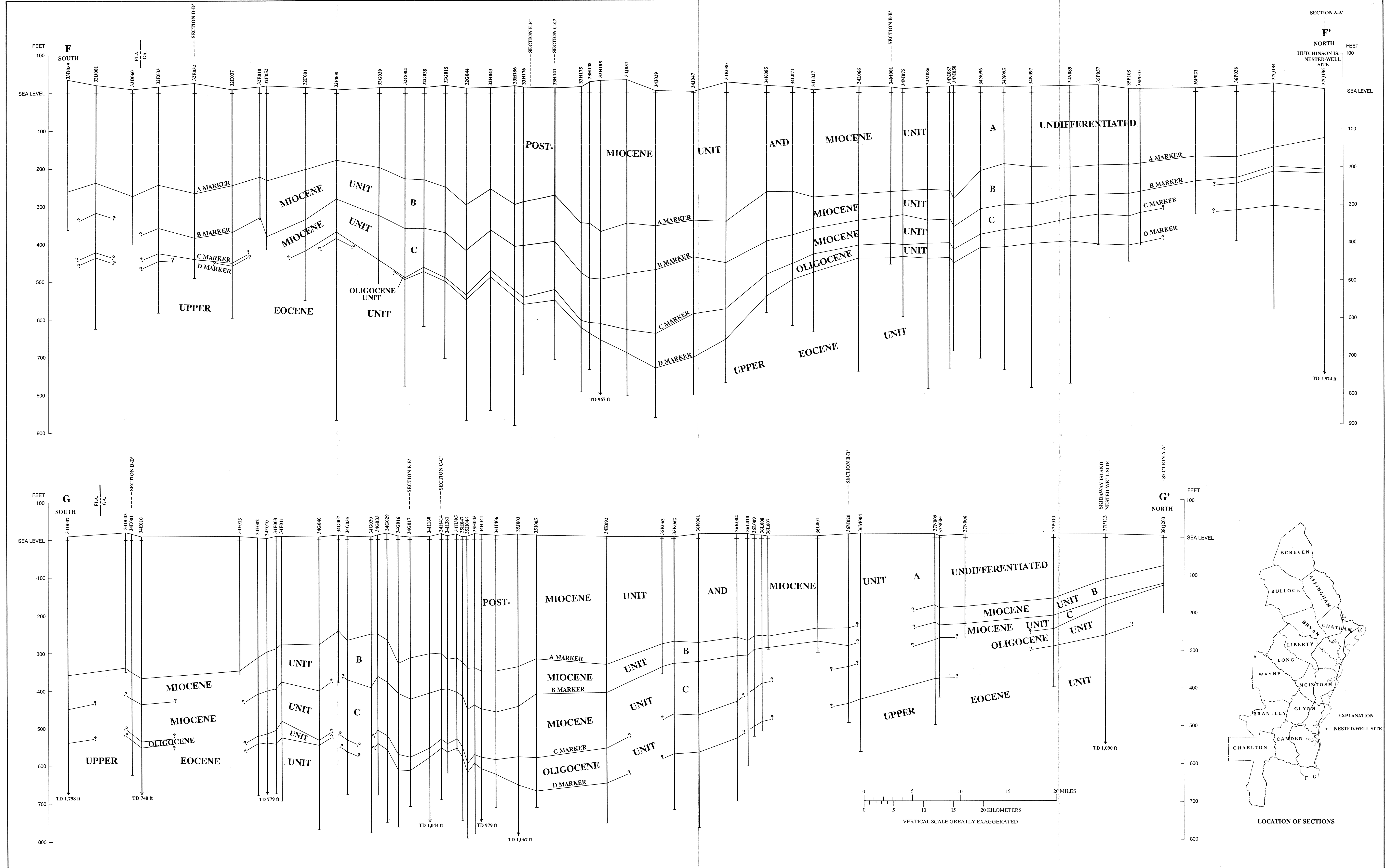
GEOLOGIC SECTIONS F-F' AND G-G', COASTAL GEORGIA
