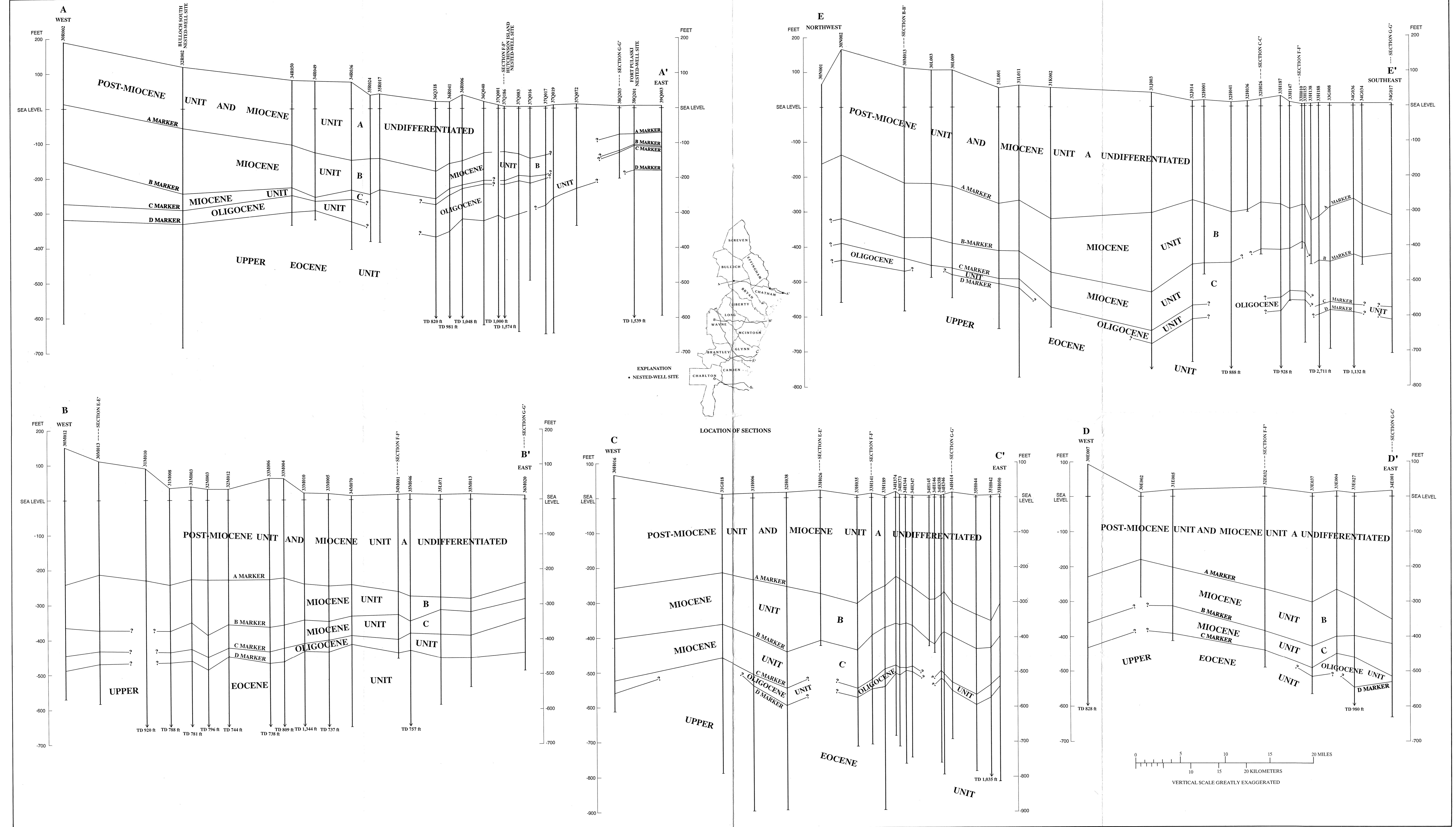
GEOLOGIC SECTIONS A-A', B-B', C-C', D-D', AND E-E', COASTAL GEORGIA
