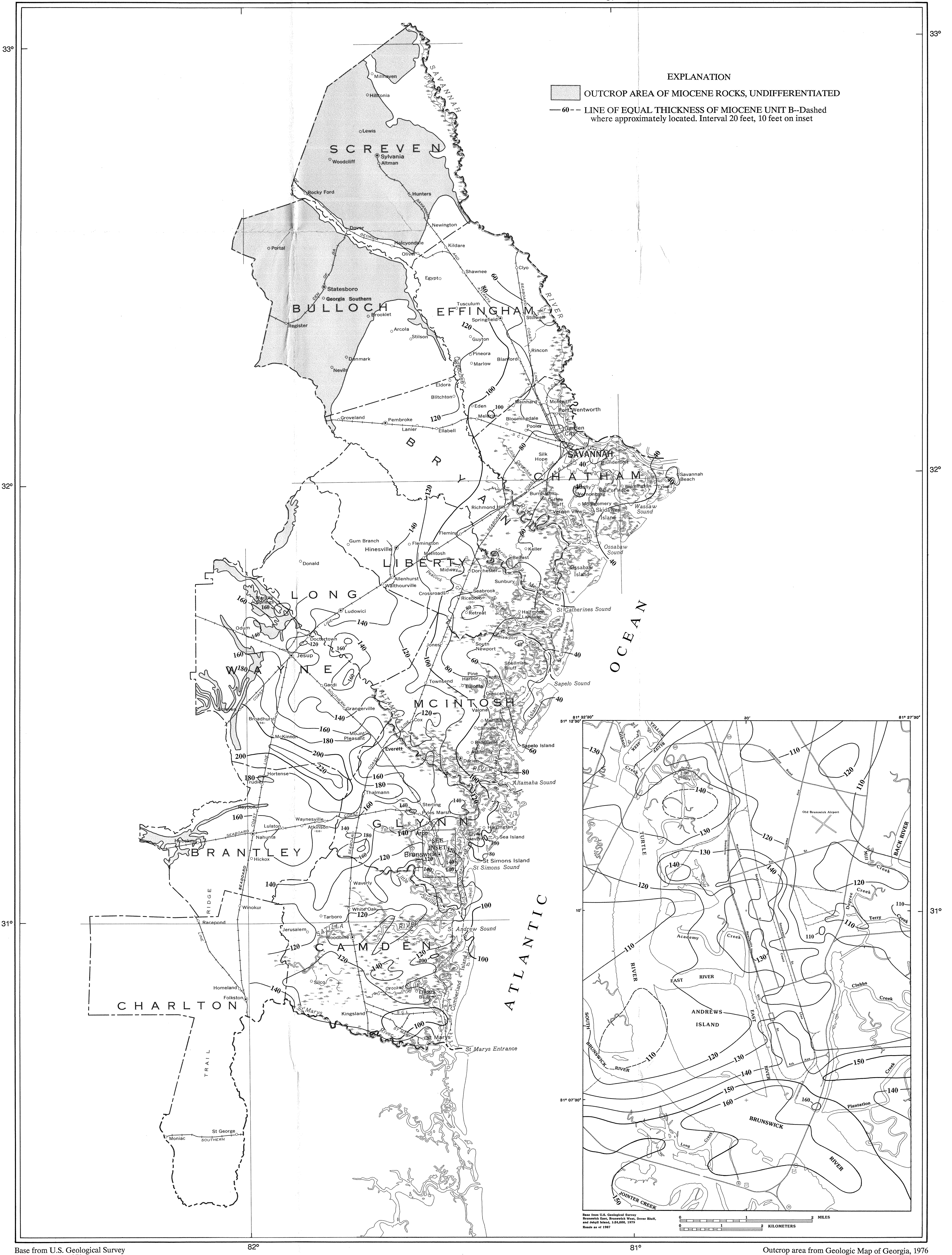
THICKNESS OF MIOCENE UNIT B IN THE COASTAL AREA, GEORGIA
